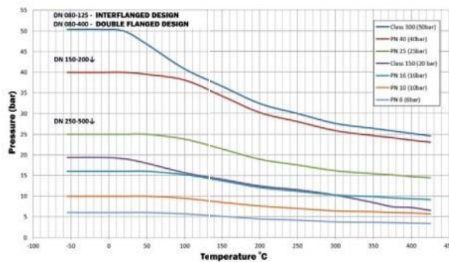
Pressure and temperature curve Body: stainless steel 1.4408
